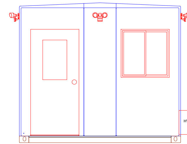
SECURE SIDE ELEVATION (Back)
