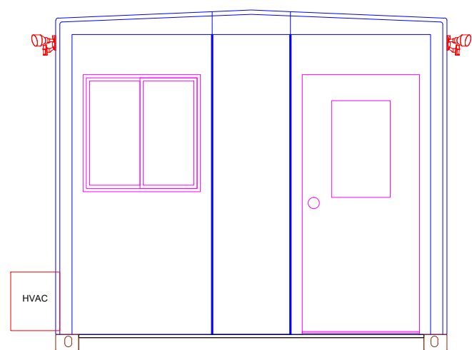
INT. ELEVATION (Facing Back)
