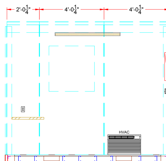
RIGHT SIDE CROSS SECTION
