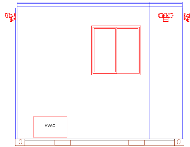
LEFT EXT. ELEVATION
