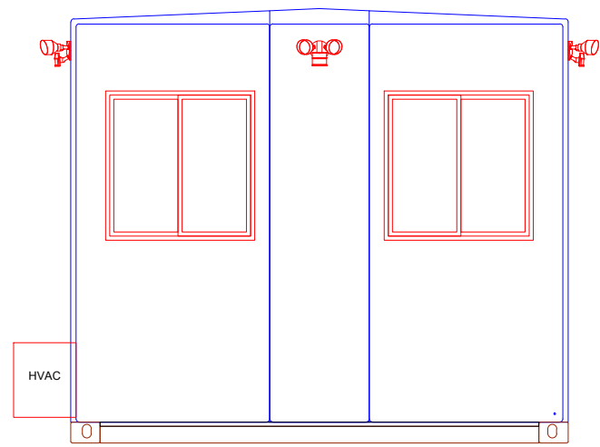
NON-SECURE SIDE ELEVATION (Front)
