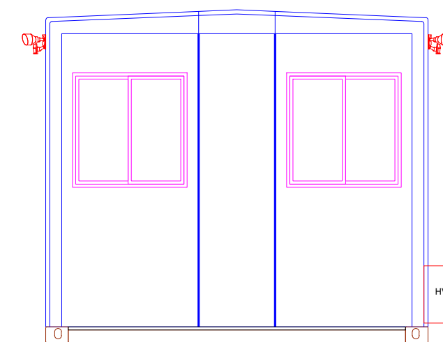
INT. ELEVATION (Facing Front)
